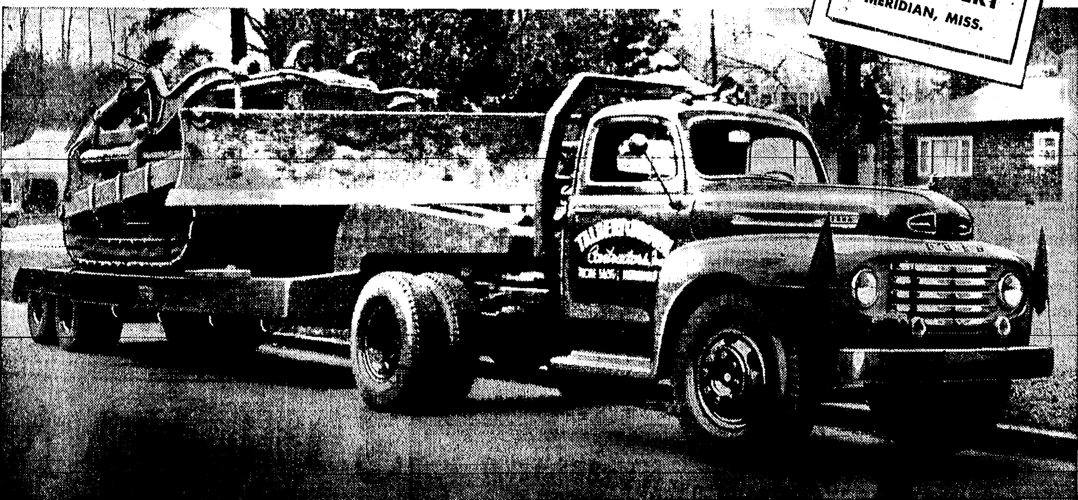
Ford Model F-8 Big Job shown has Gross Vehicle Weight rating of 21,500 lbs.; Gross Combination Weight rating of 39,000 lbs. as a tractor.
